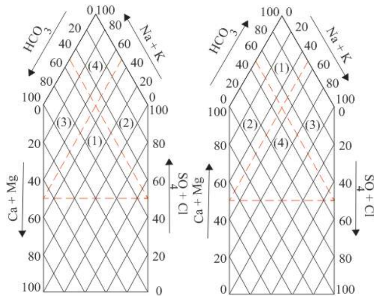
Figure (1): The Trigonal Diagram of Elhag Banaga.
