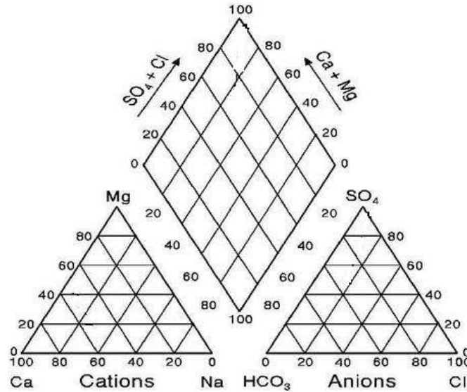
Figure (2): Piper diagram.
