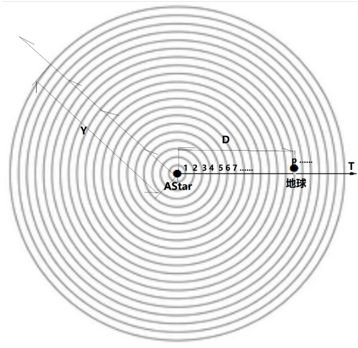
Figure 5.9: The photons continuously emitted by star AStar are grouped into successive, discrete bursts of light. Star AStar has a lifespan of Y years and is located at a distance of D light-years from Earth.
