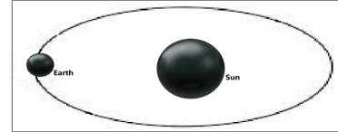
Figure 5.10: At any given moment on Earth’s orbit around the Sun, there is only one Earth and one Sun.
