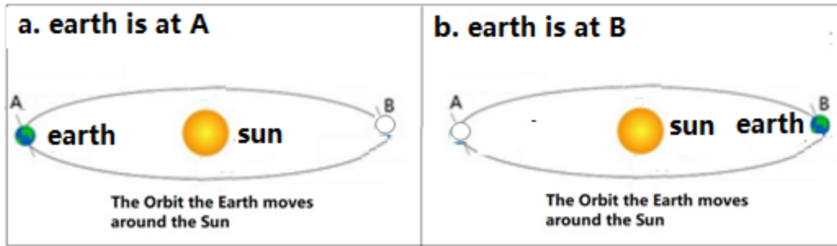
Figure 3.2: Earth's orbital space around the sun. By definition, the Earth passes through points in orbital space in turn. Left: When the Earth is located at Point A of the Earth's orbital space. Right: When the Earth is located at Point B of the Earth's orbital space.
