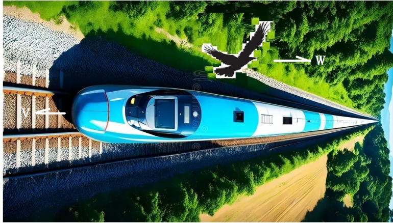
Figure 2.9: A train moving at a uniform speed v , a raven flying at a uniform speed w in the surrounding real-world environment. Please imagine that when a raven is flying in the sky, a train comes, a train leaves, or a train is moving near the flying raven as shown in the picture. Will the train have any effect on the raven's flight? Will the observation, relative calculation, imagination, etc. of the man in the train have any effect on the raven's flight? There is another lady in the train who want to keep the raven in a cage.
