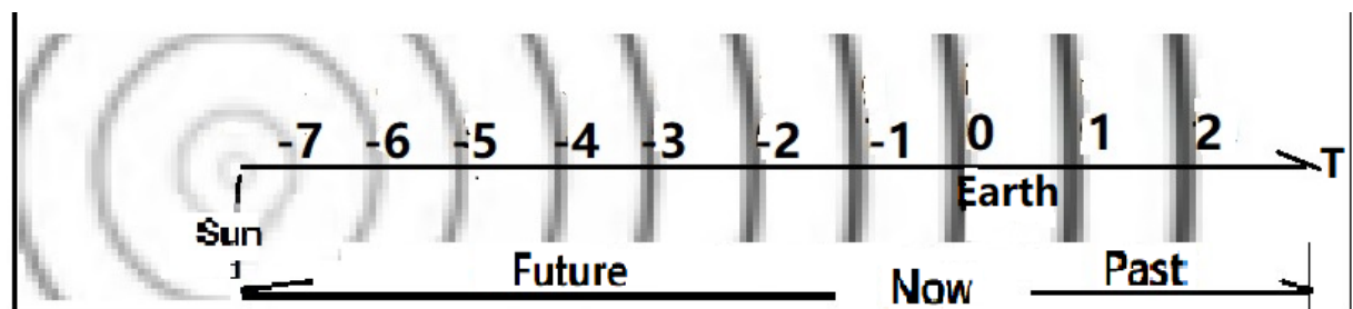
Figure 5.7: Understanding the time related to the flow of unit objects 3: The observable “past,” “Now,” and “future” of all batches of photons emitted by the Sun within 10 minutes, relative to the observer’s position on Earth, with Earth as the origin.
