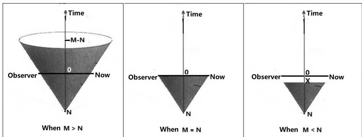
Figure 6.7: The three shapes of new light cones with the distances are N light years between the observer and the star, and the lifetime of the star is M years.
