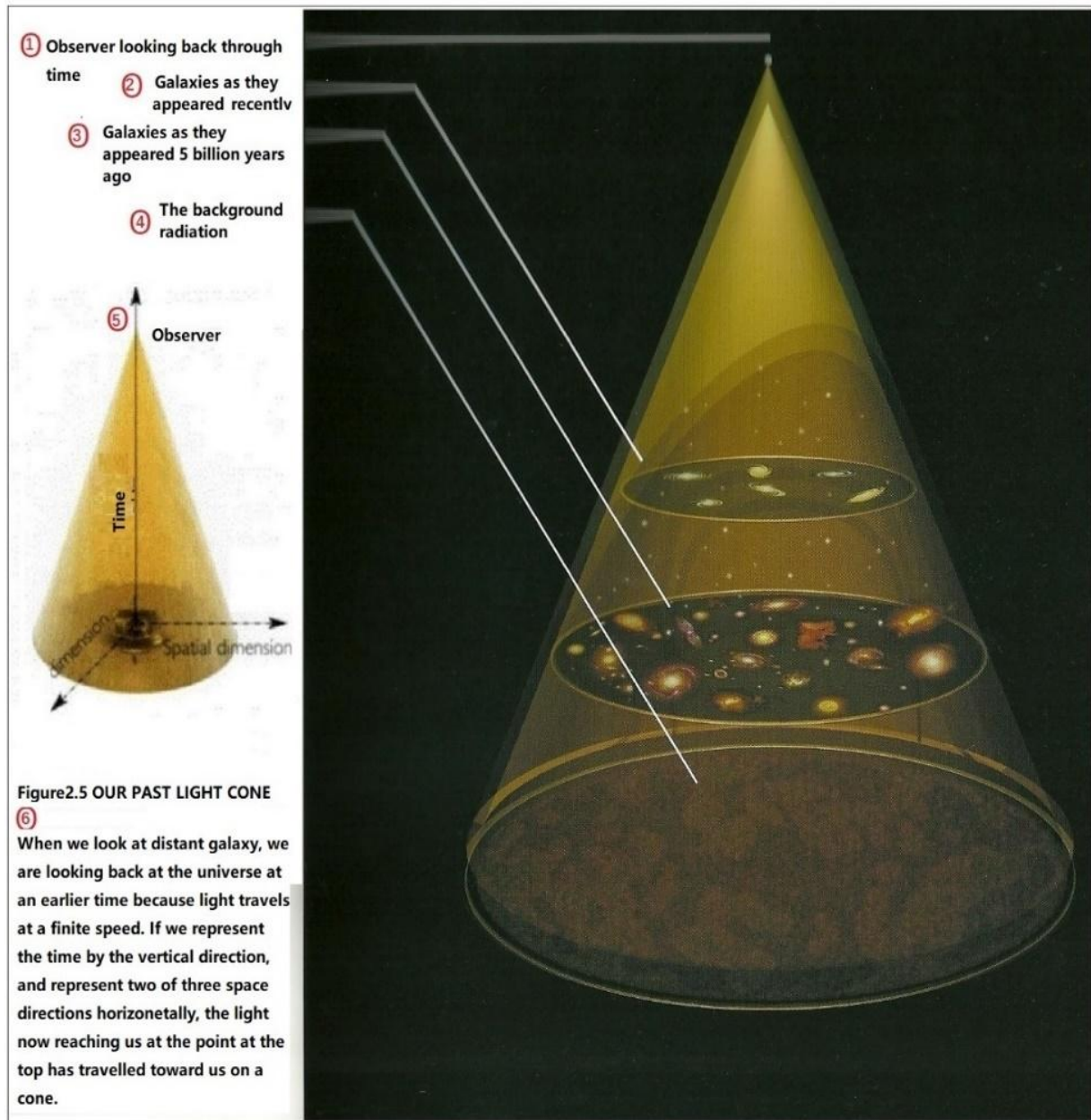
Figure 6.2: Hawking's past light cone and its interpretation from <The Universe in A Nutshell>.
