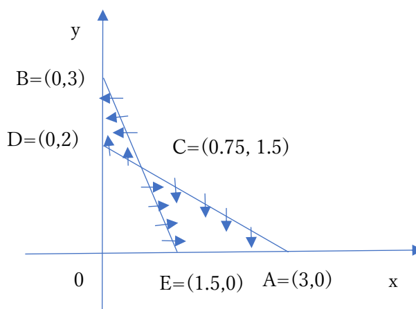
Figure 1: Two lines on which \frac{dy}{dx} = 0 or \pm\infty . On line B-E, \frac{dy}{dx} = 0 , while on line D-A, \frac{dy}{dx} = \pm\infty .
