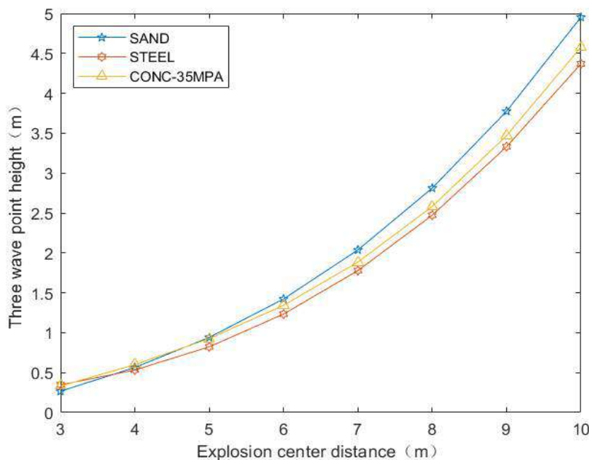
Figure 11: Comparison of three-wave point trajectory curves at different reflective interfaces
