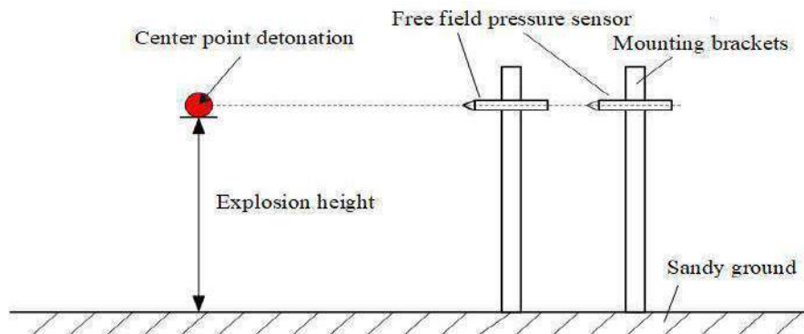
(a) The overall picture of the test physical model
