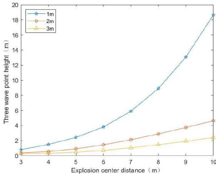
Figure 7: Comparison of three-wave point trajectory curves at different explosion heights
