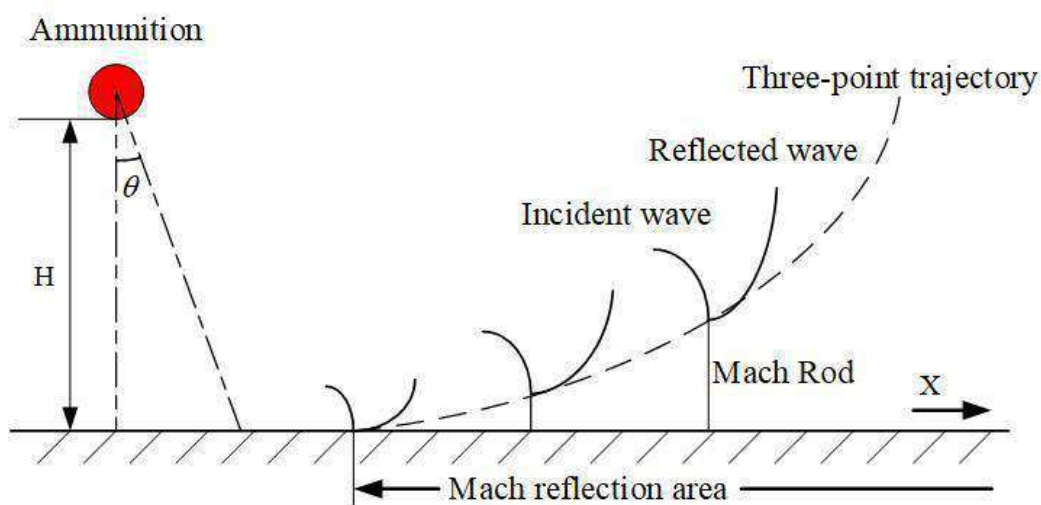
Figure 1: Schematic diagram of near-ground explosion field
