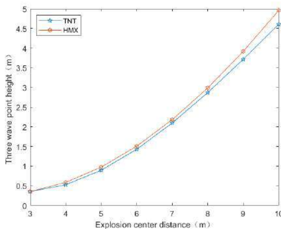
Figure 10: Comparison of three-wave point trajectory curves for different charging materials
