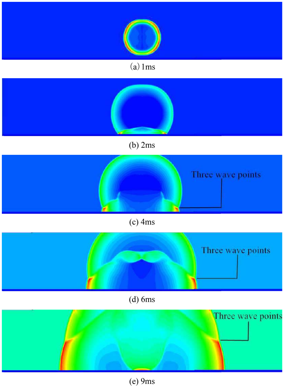
Figure 5: Shock wave pressure cloud diagram at different times
