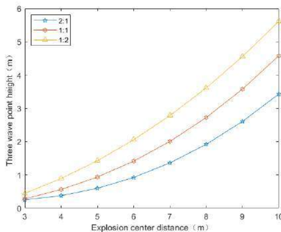
Figure 9: Comparison of three-wave point trajectory curves of different charge sizes
