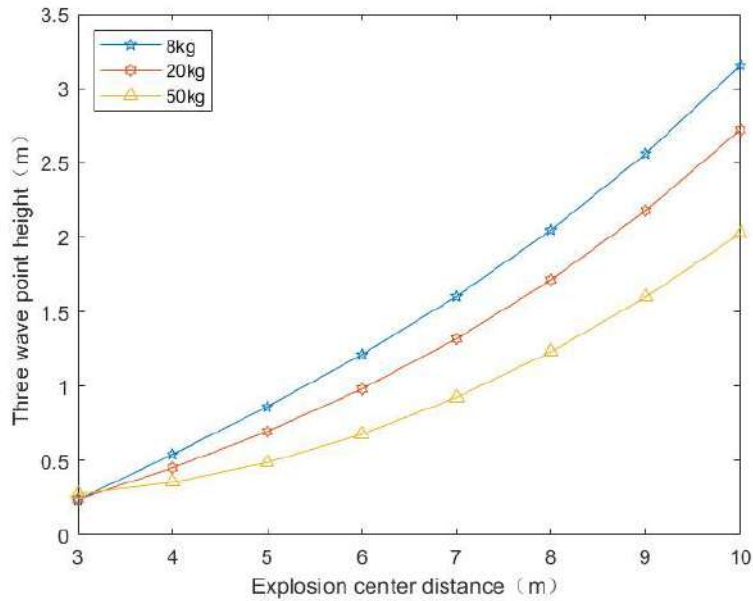
Fig. 6: The height of the three wave points varies with the burst center distance at different equivalents
