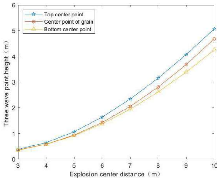
Figure 8: Comparison of three wave point height curves at different initiation points
