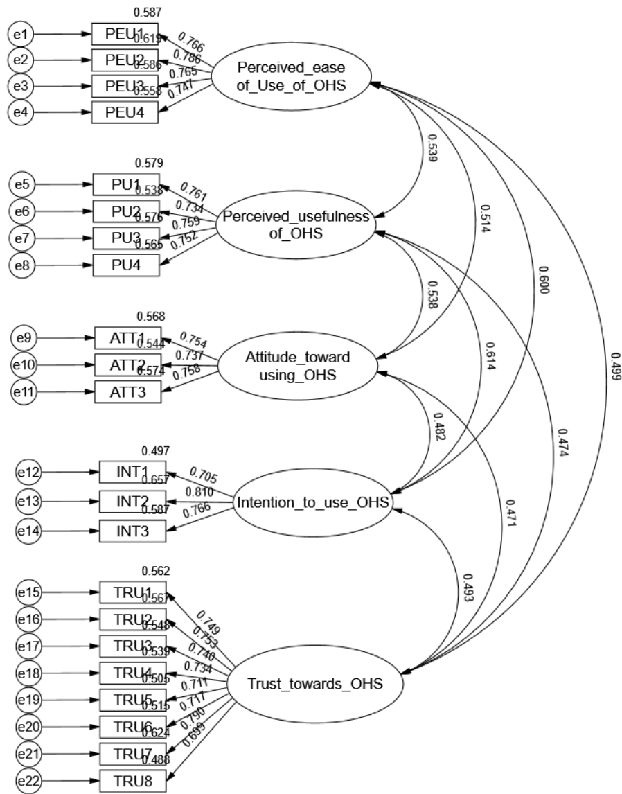
Figure 3: Measurement Model
