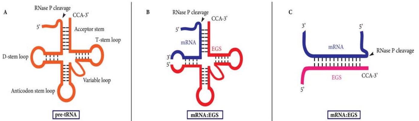
Figure 1: Substrates for bacterial RNase P and M1 RNA (A-C)
