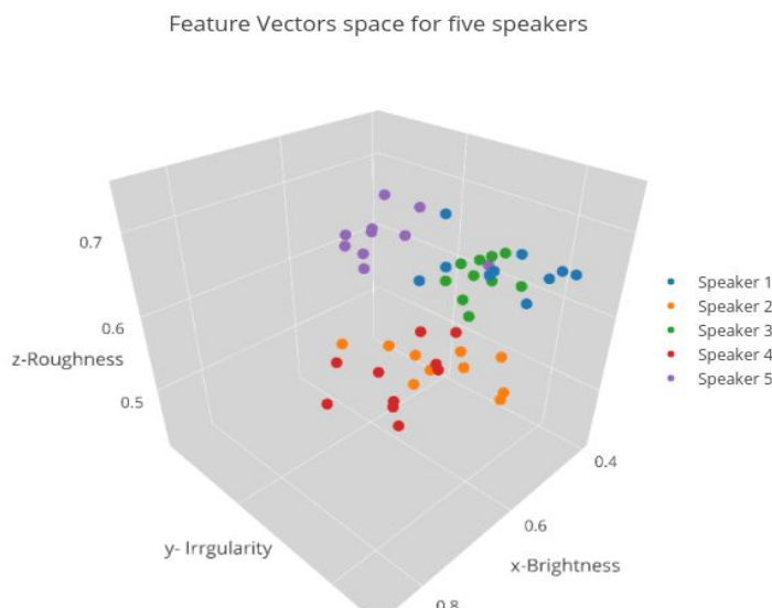
Fig. 4: Feature vectors in 3-D space for five speakers each with 10 samples
