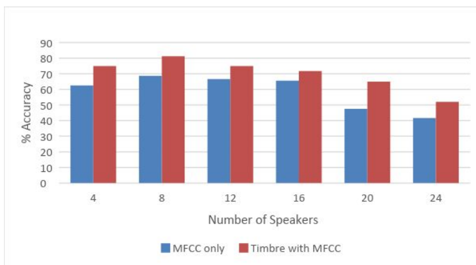
Fig. 7: Comparative identification results by Timbre features and MFCC features
