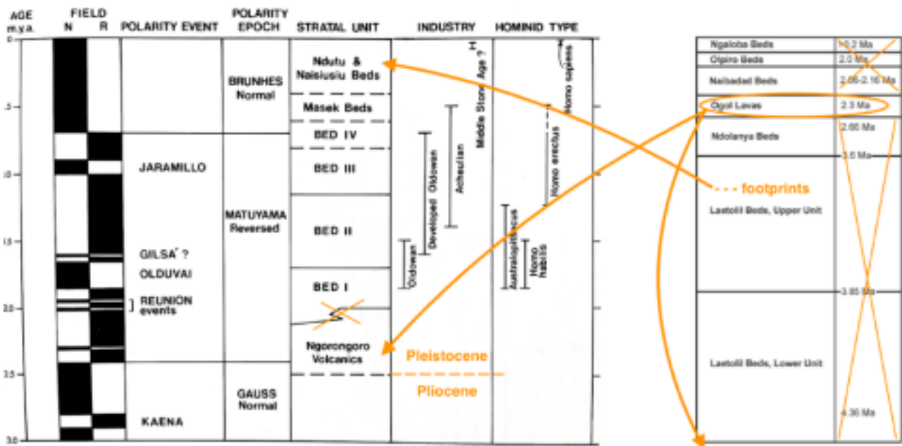
Fig. 7: Horizontal strata at Olduvai (left diagram, from 18) and Laetoli (right diagram, from 19). Hay (20) thought Ogot volcanics lie over Laetoli Beds. I think the Ogot Lavas are volcanic basement, which includes inselbergs like Namorod and Engelosin.
