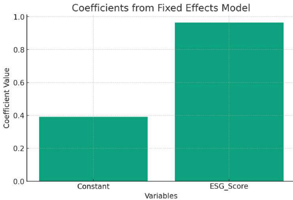
Fig. 4: Coefficient and Fixed Effect MODEL
