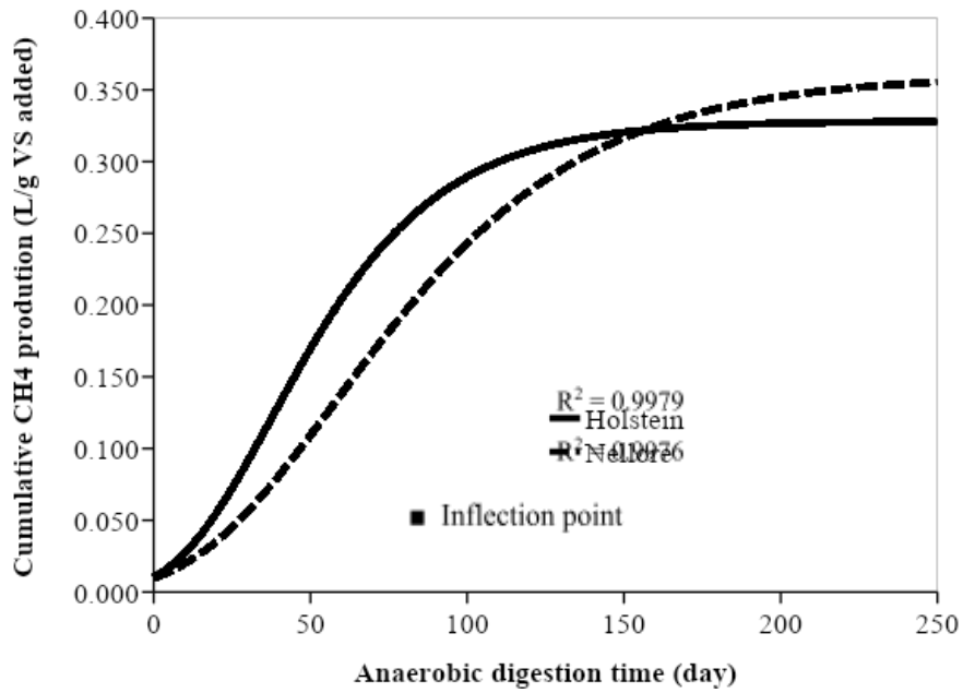
Figure 1: Cumulative CH 4 production, adjusted by the Gompertz model in anaerobic batch-type digesters supplied with manure of Nellore and Holstein cattle fed Acacia mearnsii tannins. The inflection point represents the day when the maximum point of CH 4 production occurred.
