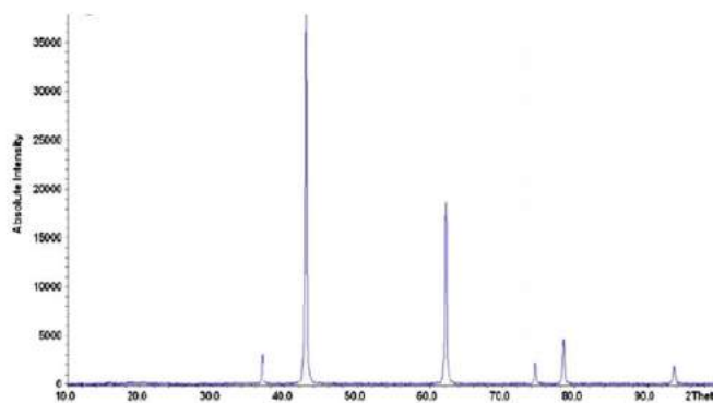
Fig.3.3: XRD analysis of presence of Nano CaO
